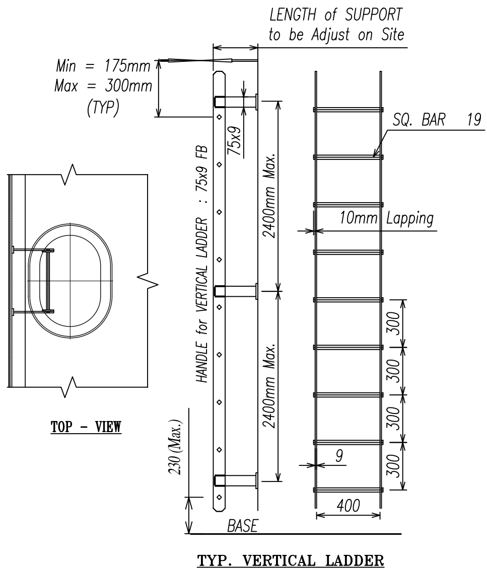
TYP. VERTICAL LADDER
